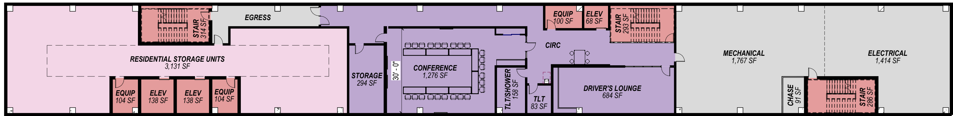
2 BASEMENT CONCEPT PLAN 1" = 20'-0"
