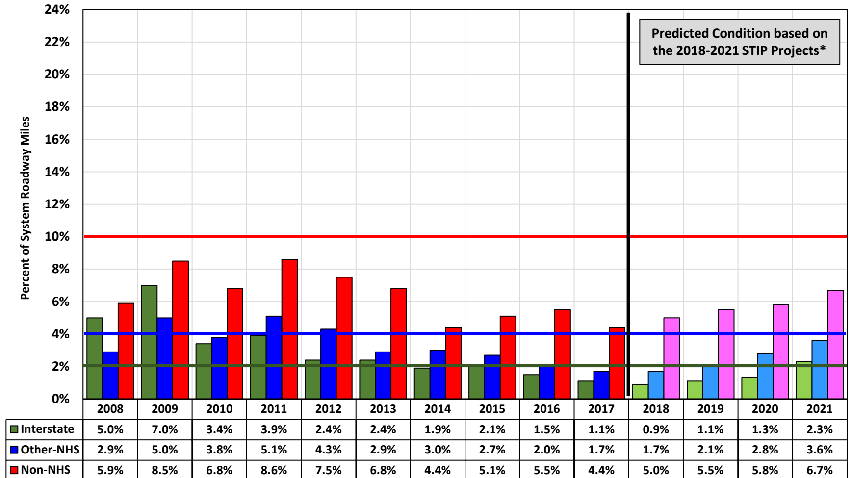
Figure 3 Statewide "Poor" Ride Quality Index (percent of roadway miles with an RQI of 2.0 or less) Actual 2008-2017, Predicted 2018-2021
