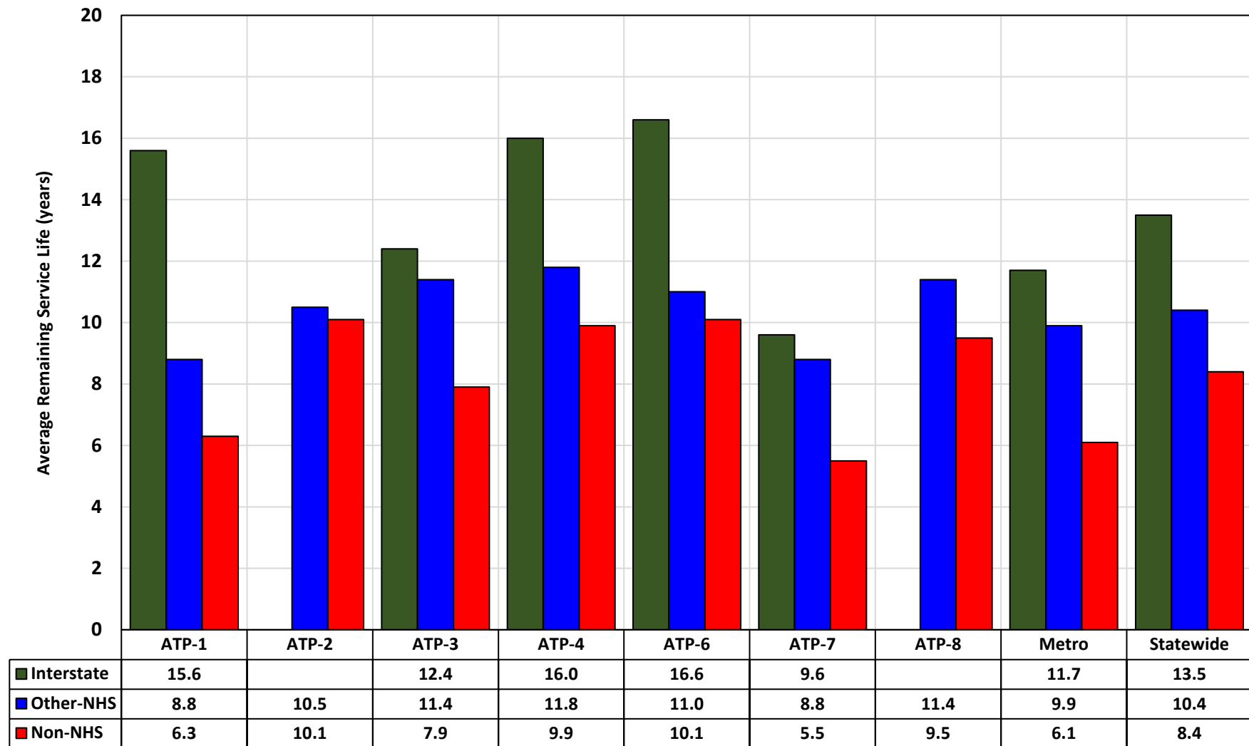
Figure 13 Average Remaining Service Life (ARSL) (years until RQI is predicted to reach 2.5, assuming no future work is done) Comparison of 2017 Data by ATP
