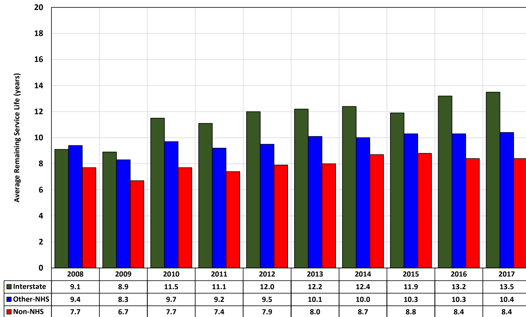
Figure 12 Statewide Average Remaining Service Life (ARSL) (years until RQI is predicted to reach 2.5, assuming no future work is done) Actual 2008-2017 data
