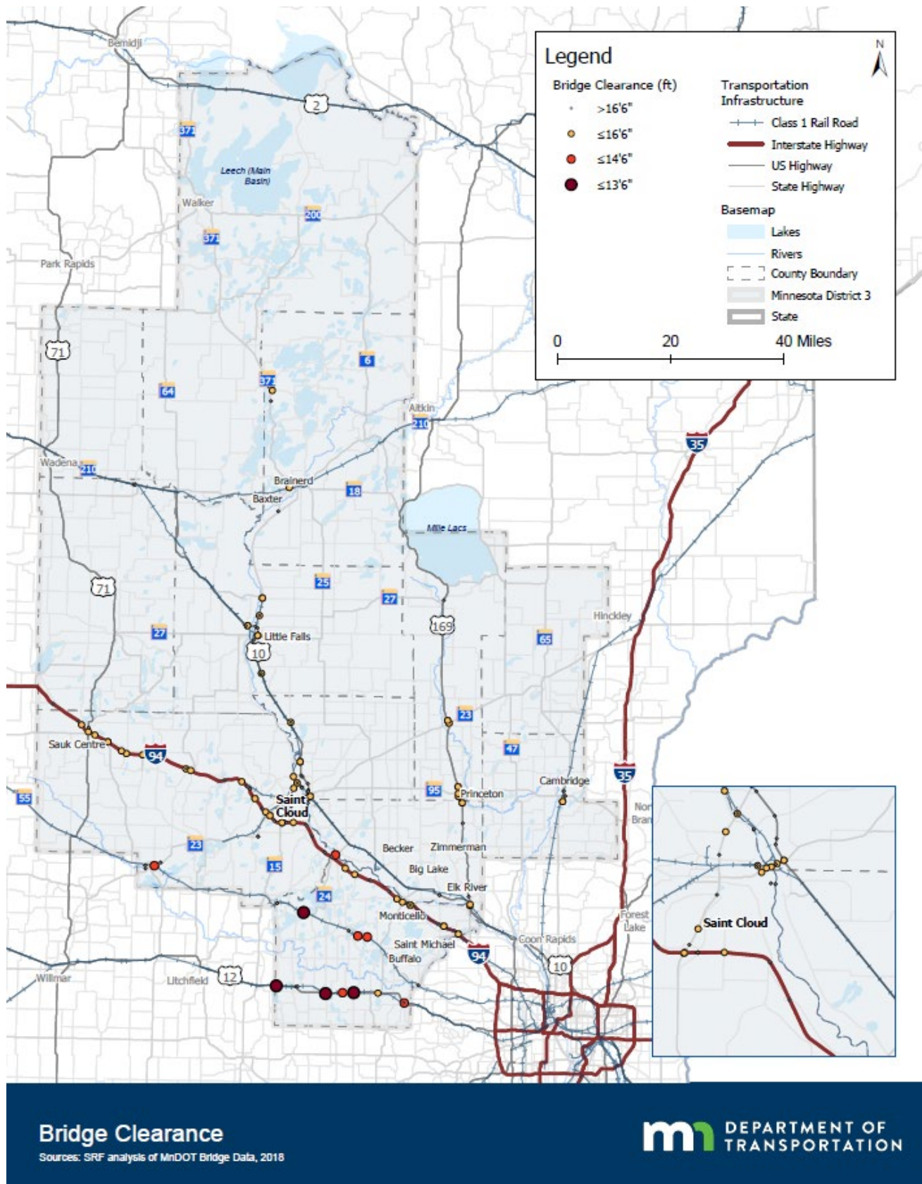
Figure 14. Bridge Clearance Restrictions
