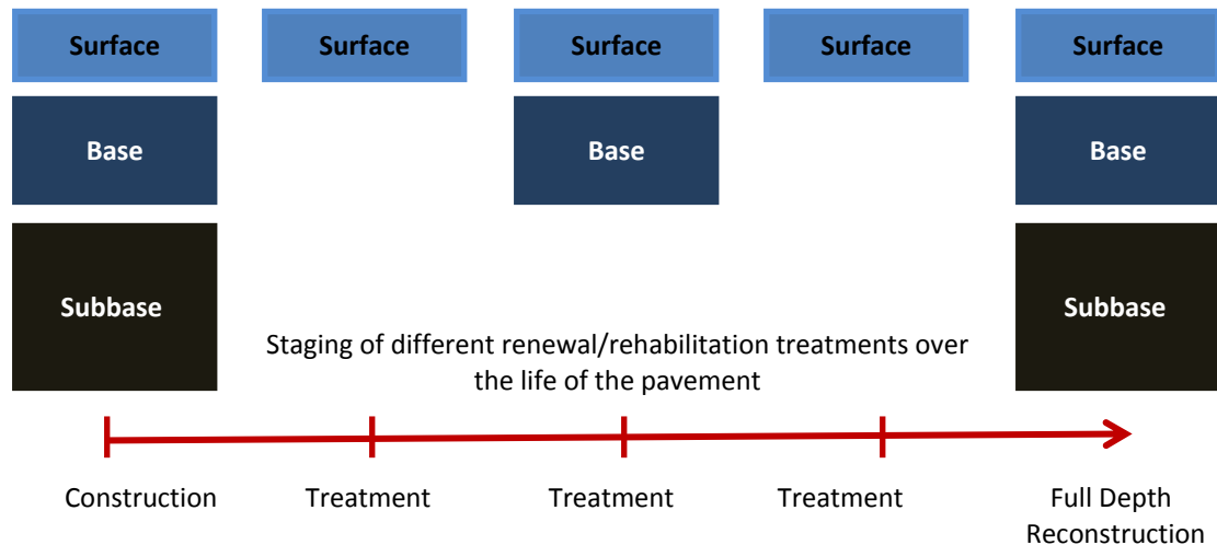
Figure 1-2 Pictorial Pavement Treatment Schedule
