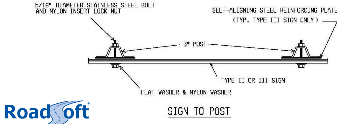
Figure 1-1 Componentized Sign Assembly
